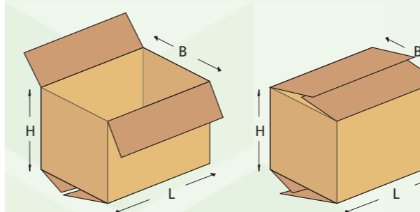
0201 - outer flaps meet
